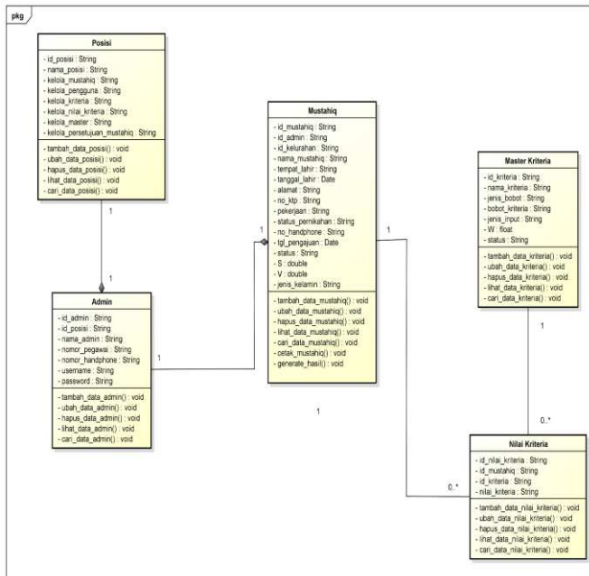
Gbr. 7. Class diagram
