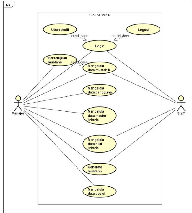
Gbr. 4. Use Case Diagram
