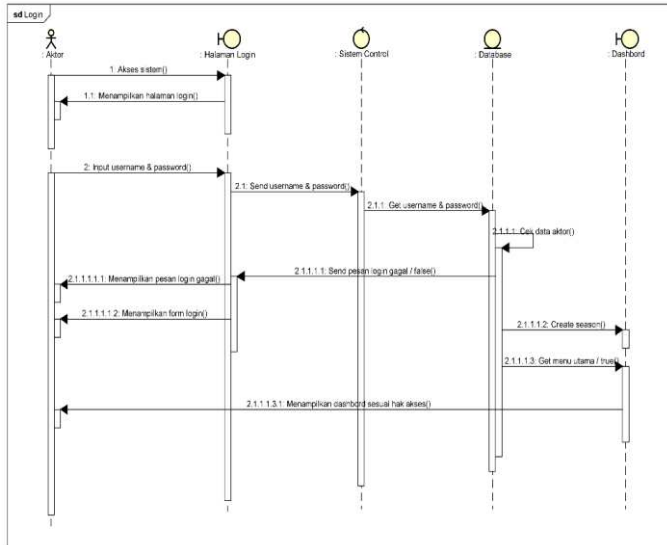
Gbr. 6. Sequence diagram
