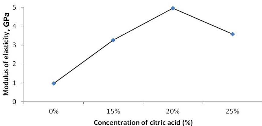
Figure 4 Modulus of elasticity from particleboard.
