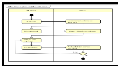
Gambar 2. Activity Diagram Registrasi Ahli waris
