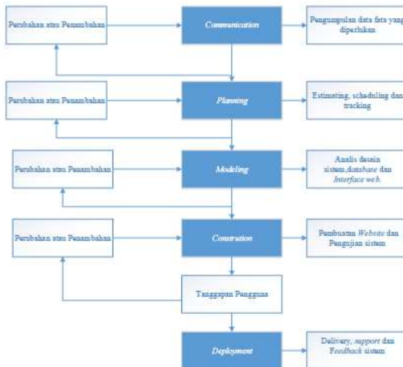
Gambar. 1. Fase Deployment
