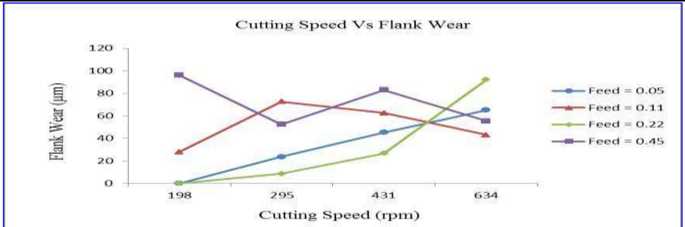
Fig. 6.9 Variation of Flank Wear with Cutting Speed
