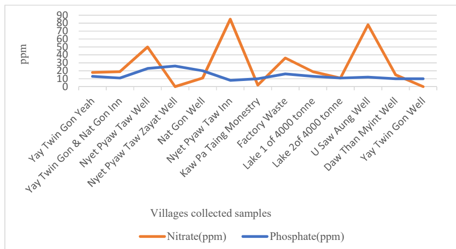
Figure 3: Concentrations for nitrate and phosphate in selected villages (source: AMTT Co., Ltd) Conferring to the report of Advancing Life and Regenerating Motherland, chlorine, nickel, BOD, and COD are found as higher levels and can impact toxic to freshwater fishes.
