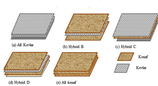
Figure 3. Configuration of Kevlar and Kenaf layer [16]
