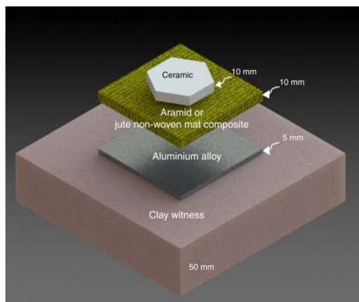
Figure 12. Schematic of a Multilayer Armour system with thickness layers [26].
