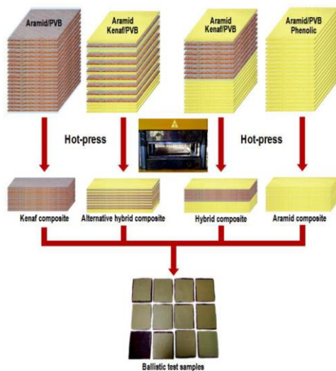
Figure 2. Kenaf/Aramid/PVB composite specimen prepared using hot press [15].
