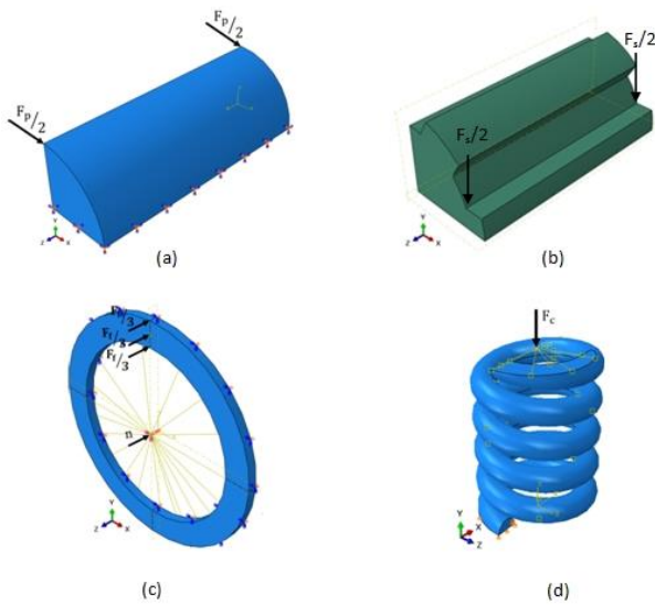
Figure 2. Applied forces at on (a) shaft (b) spline (c) friction plate (d) spring.
