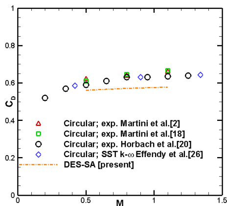
Figure 4. Discharge coefficient.
