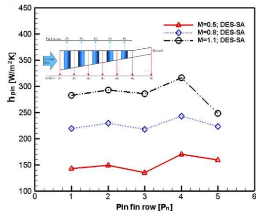
Figure 3. Pin-fin HTC.
