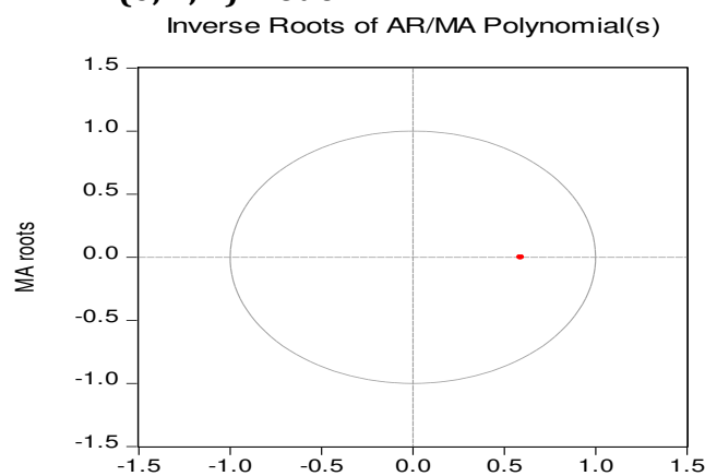
Figure 2: Inverse Roots
