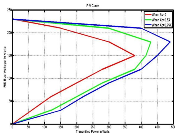
Fig.7 P-V Graph
