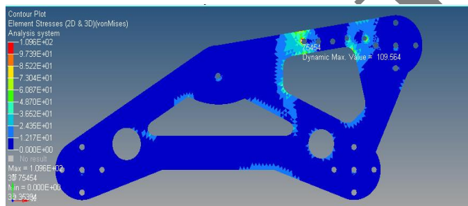
Fig 16. Stresses in the gripper after optimization
