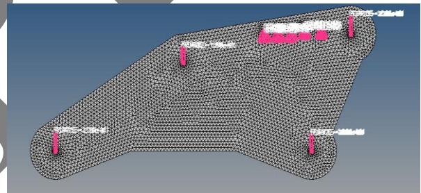
Fig 7. Boundary conditions applied.
