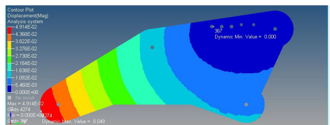
Fig 8. Before optimization the gripper displacement.
