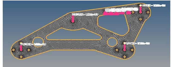
Fig 12 Gripper after the remove of material.
