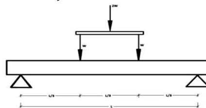
Figure No. 2. Typical Two Point Loading Arrangement
