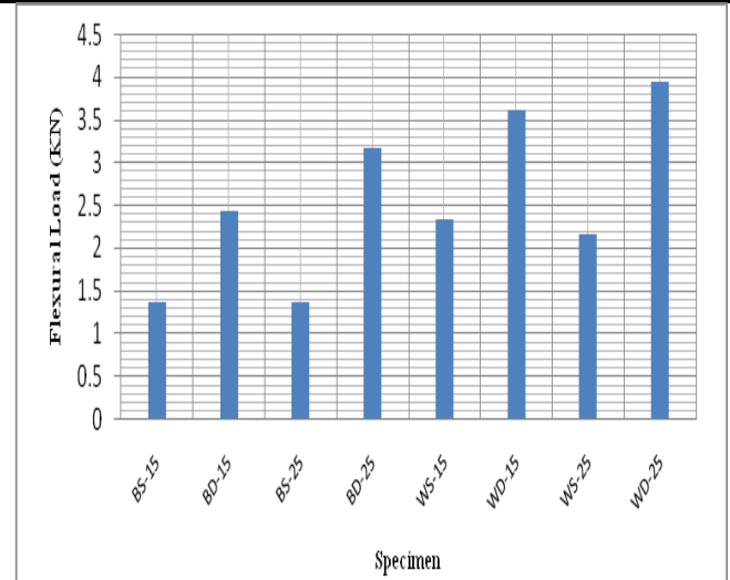
Graph No.2.28 Days Curing Flexural Load Carrying Capacity
