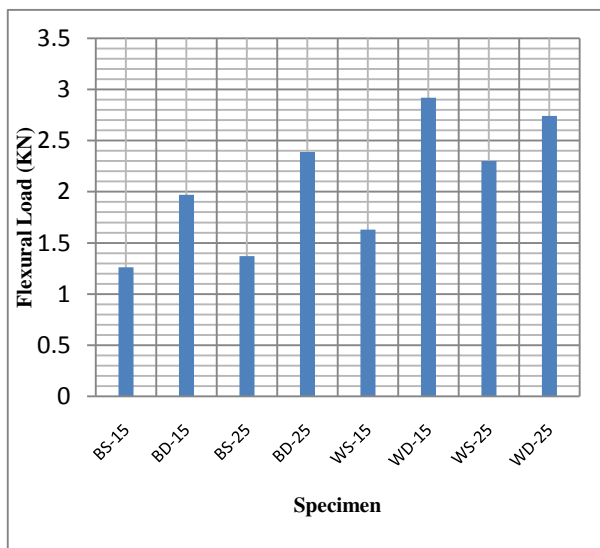
Graph No.1. 7 Days Curing Flexural Load Carrying Capacity
