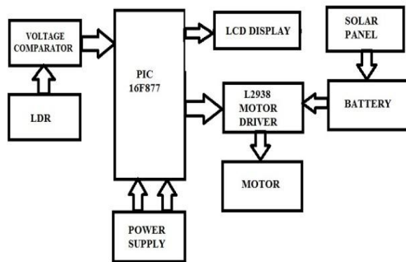
Fig.5. Schematic of diagram MPPT system.
