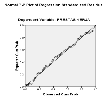
Gambar V.1 : Grafik Normal Probability P-Plot
