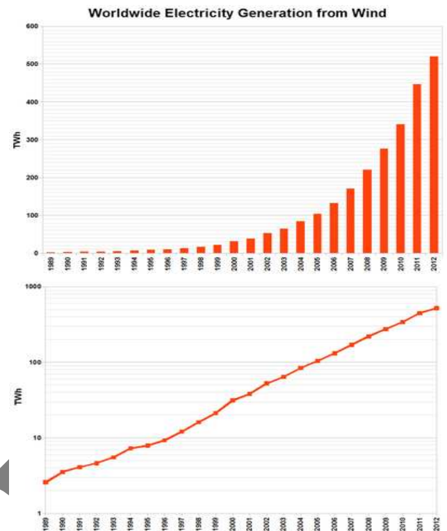
Figure 3: Worldwide wind generation up to 2012 (Source EIA, January 2015).
