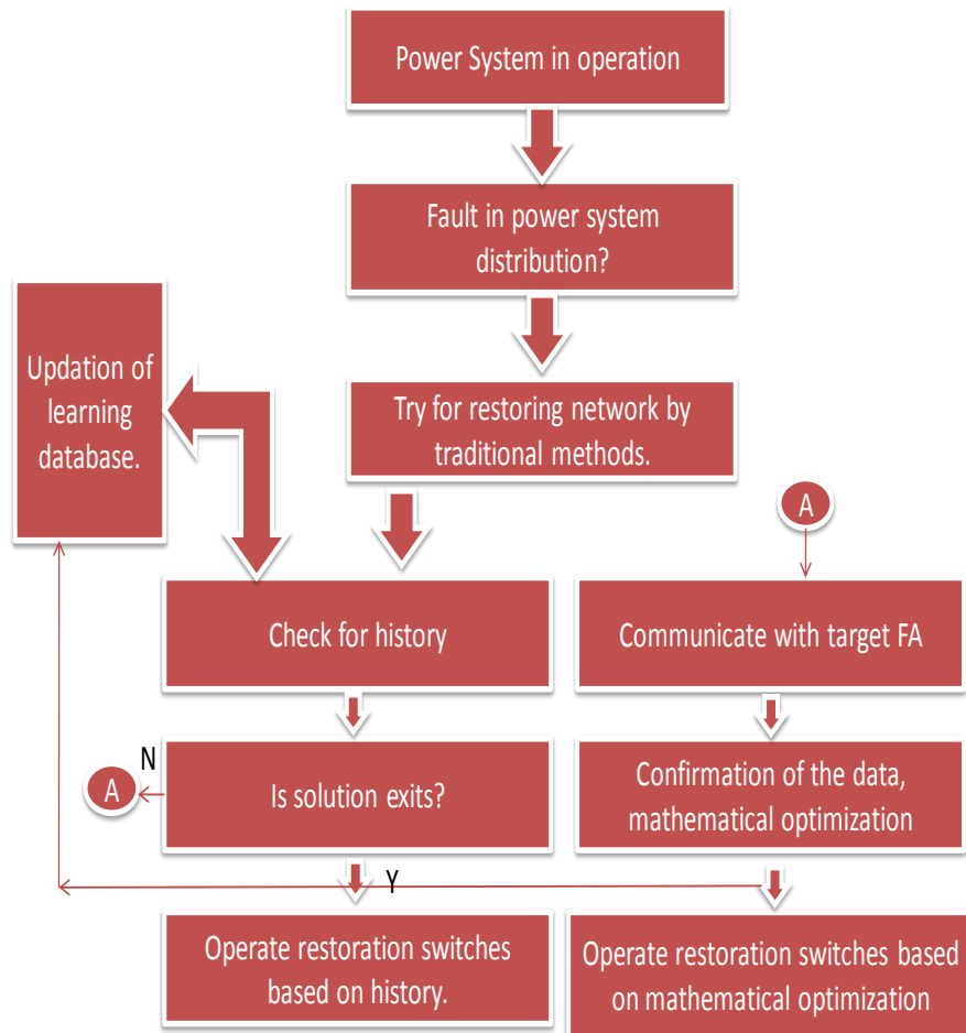
Fig.1 PROPOSED SYSTEM FOR LEARNING ALGORITHM
