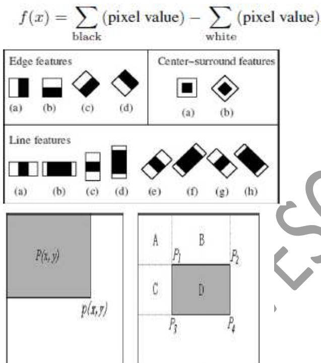
Fig.2: Extended set of Haar-like Feature Fig.3: Integral Image
