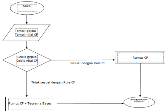
Gambar 8. Flowchart
