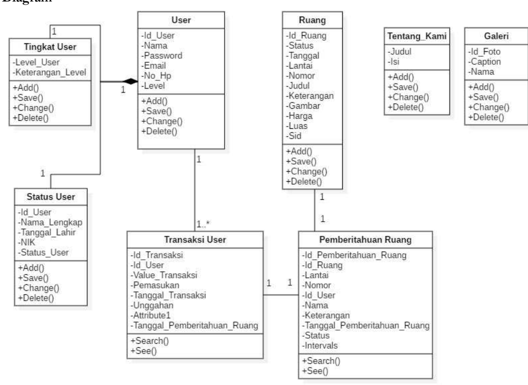
Gambar 4. Class Diagram
