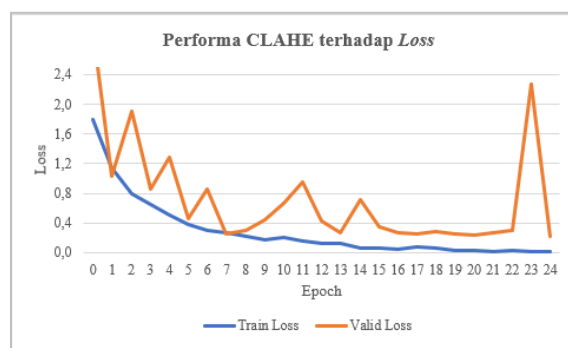
Gambar 8. Performa CLAHE terhadap loss
