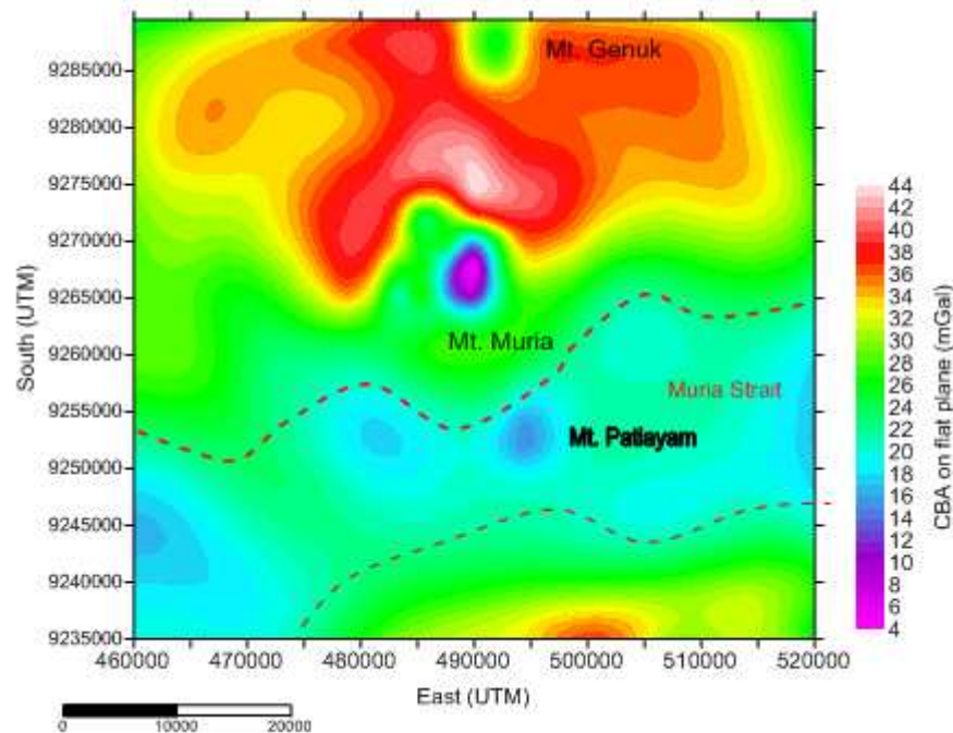
Figure 4. CBA contour on the flat plane
