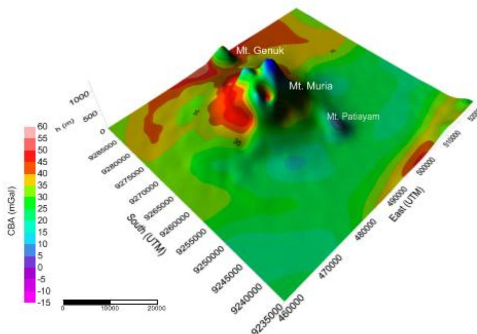
Figure 3. Topographic map overlay CBA contour in the UTM coordinate
