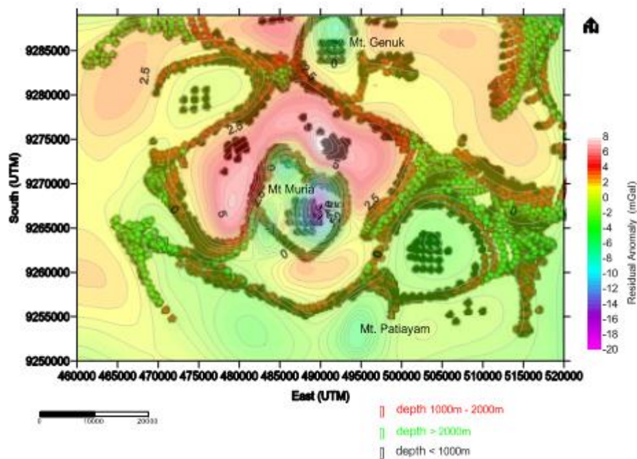
Figure 6. Residual anomaly overlay Euler deconvolution index 0
