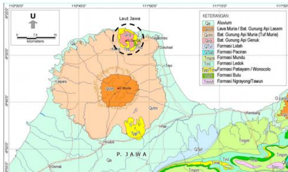
Figure 1. Geological map of Muria Peninsula (Suwarti & Wikarno, 1992)
