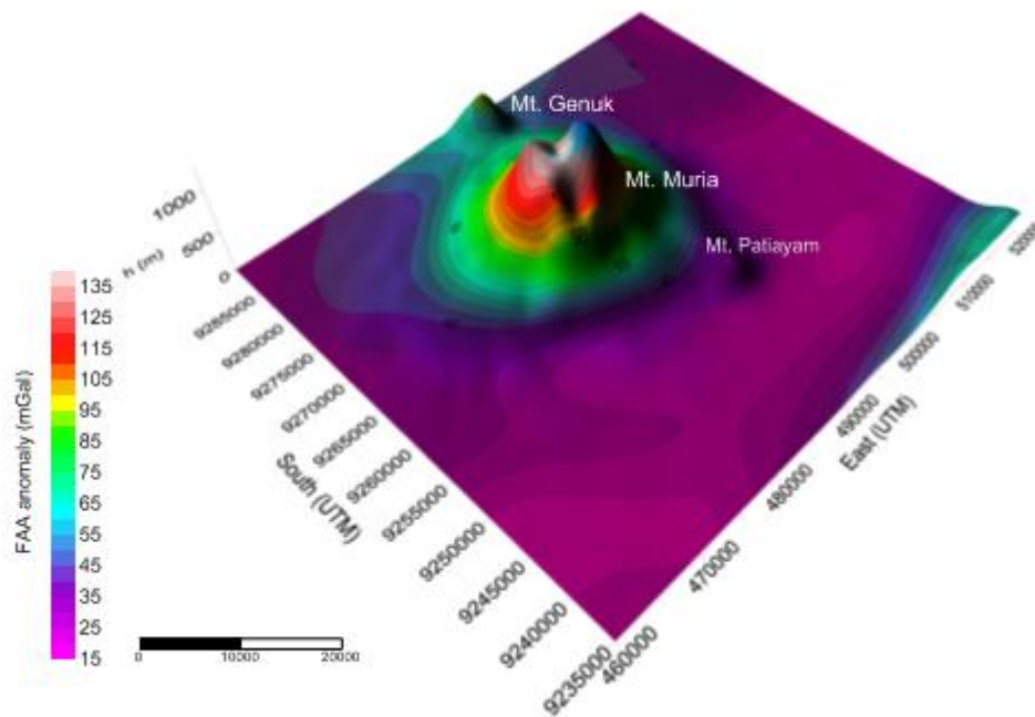
Figure 2. Topographic map overlay FAA contour in the UTM coordinate
