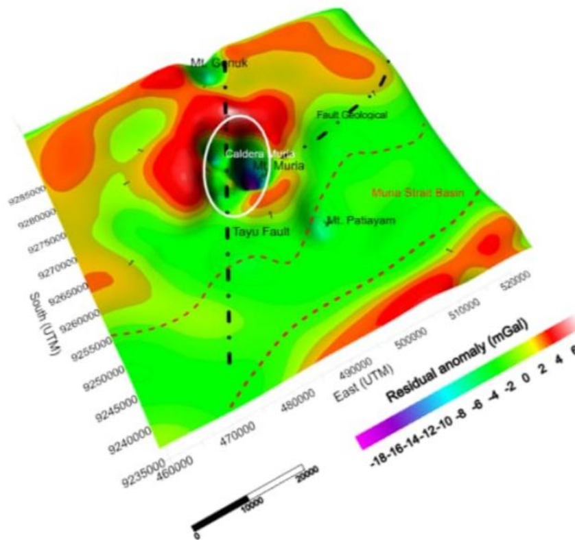
Figure 5. 3D Residual anomaly contour on the flat plane
