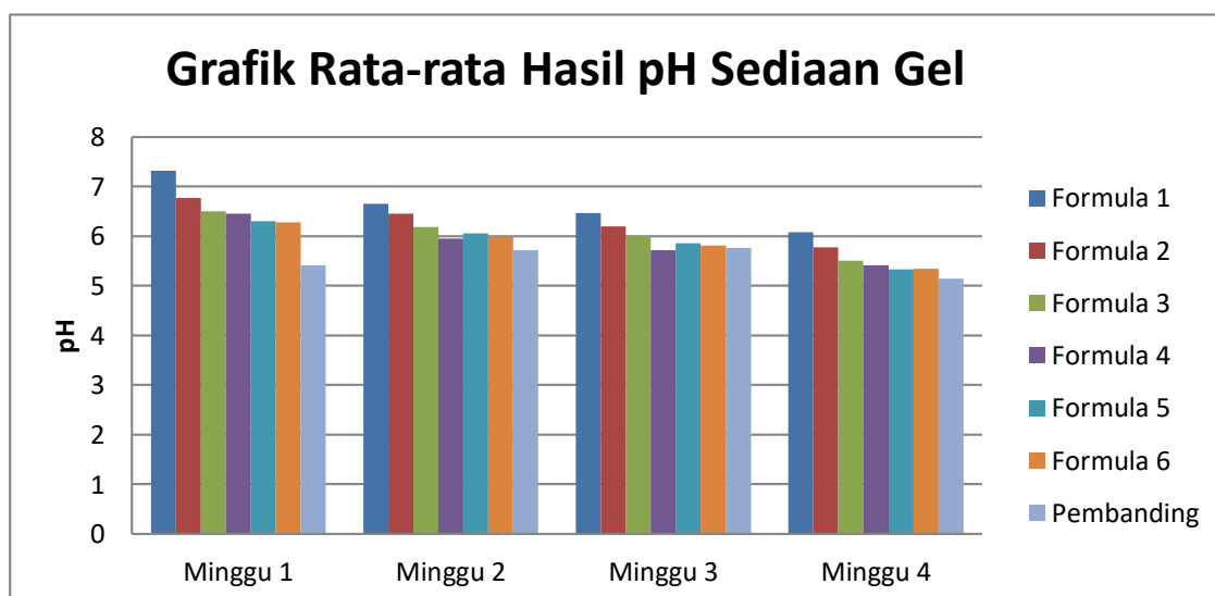
Gambar.2 Hasil pH
