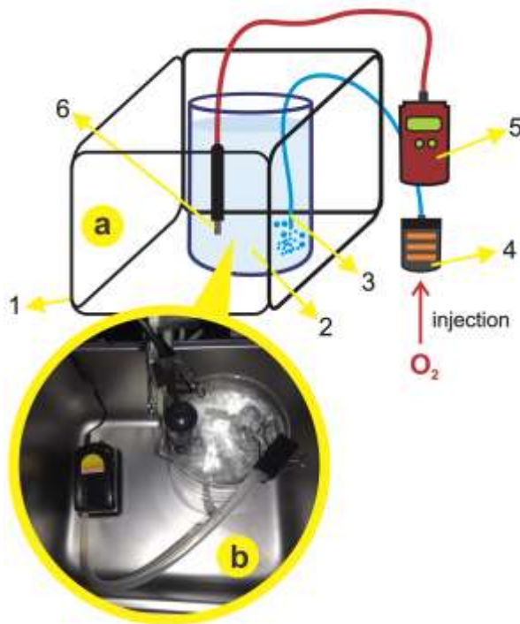
Figure 1. Full schematic illustration of simple water bath reactor (a) and real condition of the lab-experiment (b), respectively; composed by (1) reactor, (2) beaker glass 1 L, (3) aerator hose, (4) aerator, (5) DO meter, and (6) sensitive stick of DO meter.
