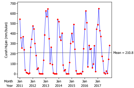
Gambar 4. Time Series Plot Curah Hujan di Pacet
