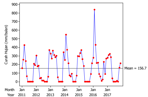
Gambar 5 Time Series Plot Curah Hujan di Mojosari
