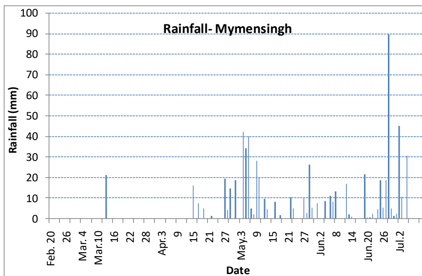
Fig.2. Rainfall pattern during crop-season in the study area
