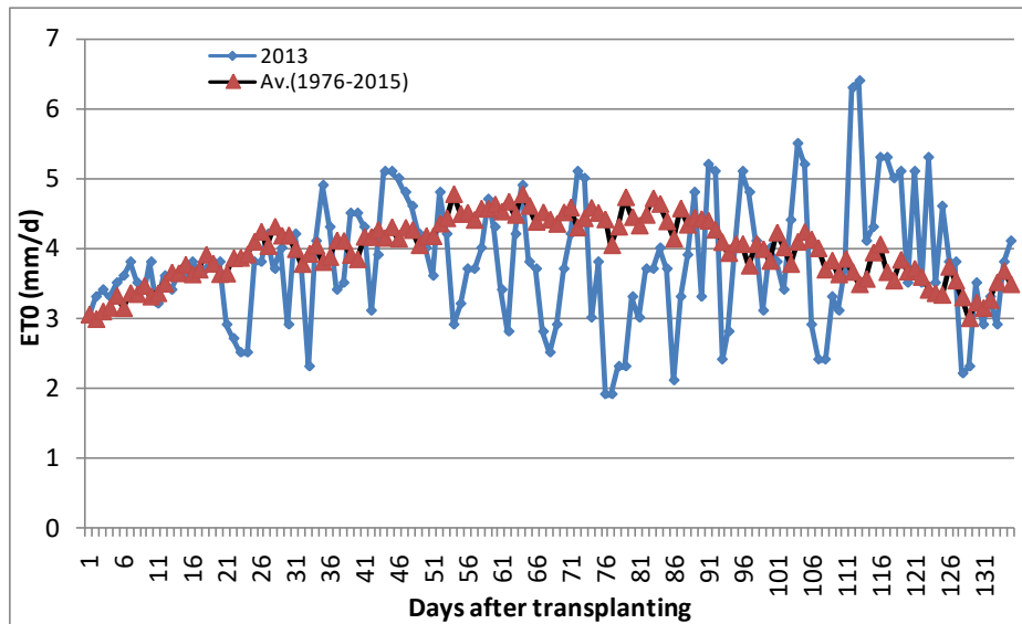
Fig.1. Crop-season and long-term ET_0 pattern of the study area
