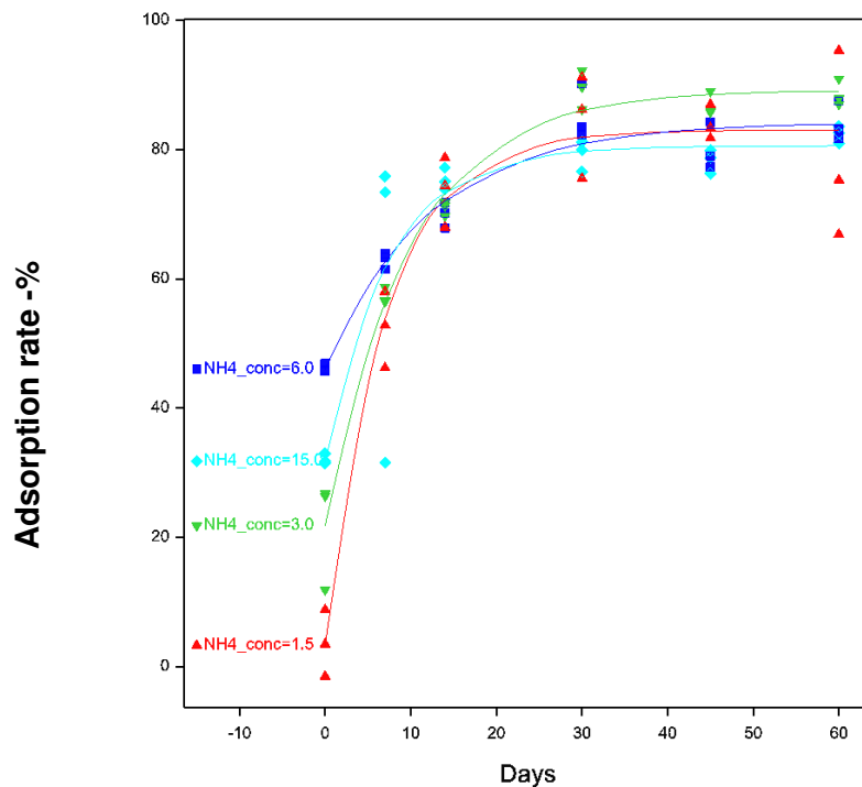
Figure 4. G30 ammonium-N adsorption capacity. Adsorption rate/submersion time.
