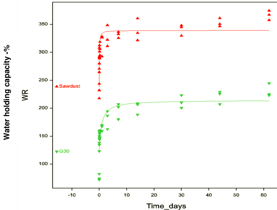
Figure 2. Water holding capacity of both woodchip types measured over a submersion period of 62 days. Both curves do not start at 0 due to the capacity of the woodchip to instantly entrain water within its matrix. This water was not considered as adsorbed.
