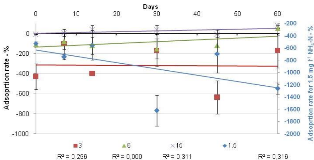
Figure 3a. Sawdust ammonium-N adsorption rate. The treatment at 1.5mg l -1 concentration was plotted in secondary axis to facilitate the observation and performance of the other three treatments.
