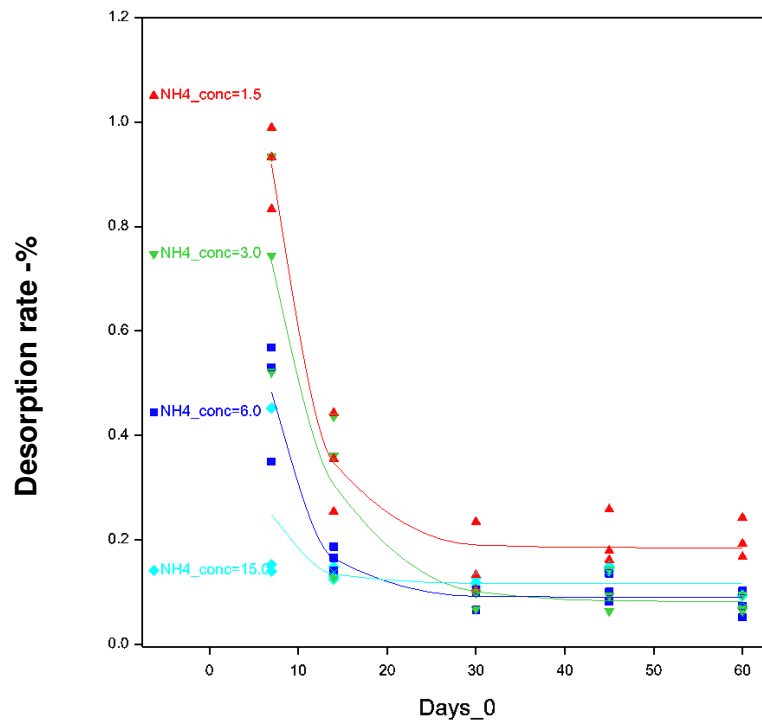
Figure 5. G30 ammonium-N desorption capacity. sorption rate/submersion time. Desorption rates at T0 for all concentrations were not included in the graph due to extremity with values that made the observation of the plotted data not clear.
