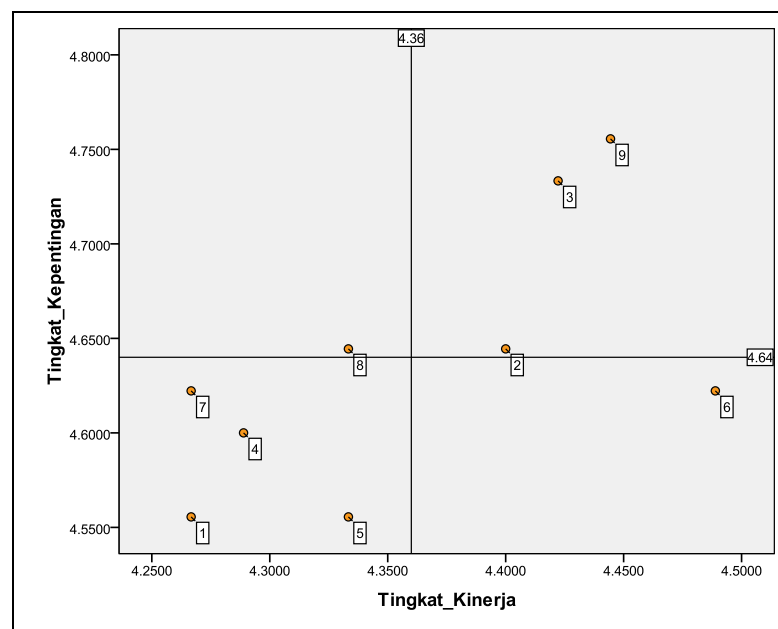
Gambar III.1 Diagram Kartesius
