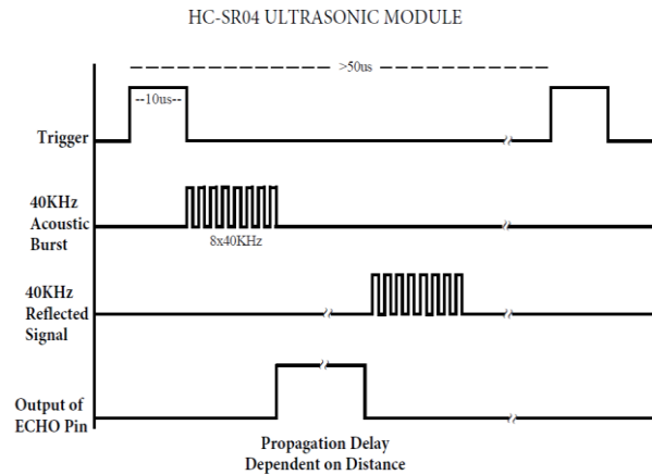
Gambar 2.5 Diagram waktu sensor HC-SR04 ( Electfreaks,2011 )
