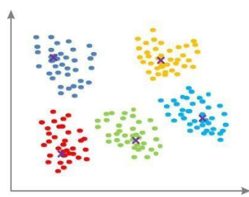
Gambar 1.1 Algoritma K-Means
