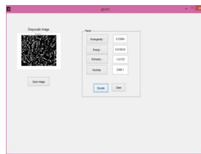
Gambar 4.3. GUI GLCM
