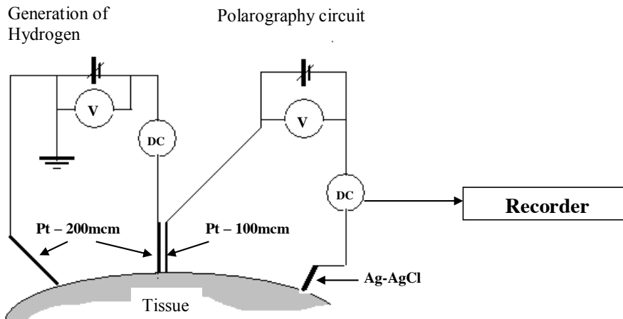
Fig.1. Principal scheme of the hydrogen electrochemical generation method measuring of the local blood flow in the tissue. Notations: V – voltage measurer, DC – direct current measurer, Pt-200µm and Pt-100µm - 200 and 100 µm diameter platinum wires, Ag-AgCl – reference electrode of chlorinated silver. See the description in the text.
