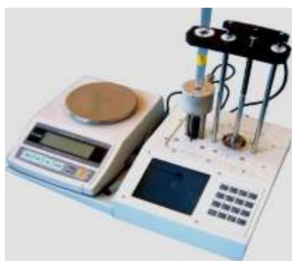
Fig. 1. Device for Electromagnetic Evaluation of the Electrical Conductivity of Powdered Materials for Lithium Batteries
