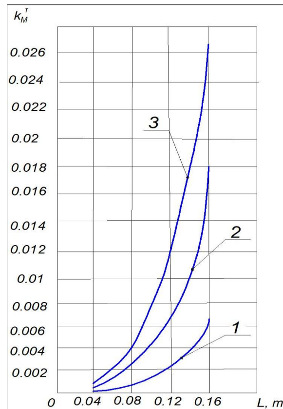
Fig. 10. Graphs of changes in the coefficient k_M^{\tau} in the model depending on the length of the section L , m: 1 - rigidity of the support structure with c = 35 \text{ N/m} ; 2 - rigidity of the support structure at c = 100 \text{ N/m} ; 3 - rigidity of the security structure at c = 150 \text{ N/m}
