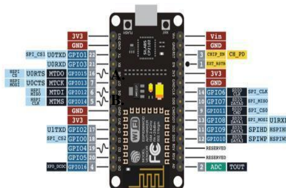
Gambar 3 Pinout NodeMCU ESP8266
