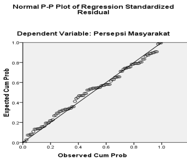
Gambar 1 Normal P-Plot
