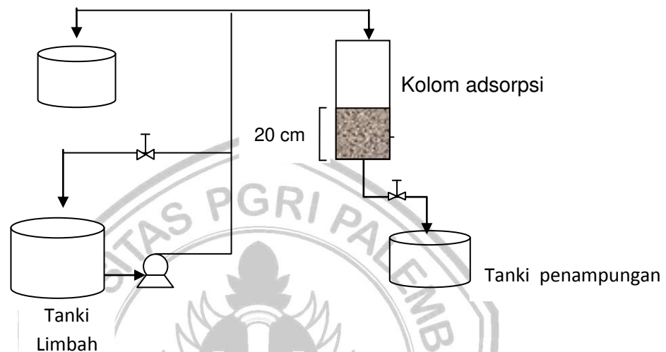
Gambar 1. Skema Alat Adsorpsi
