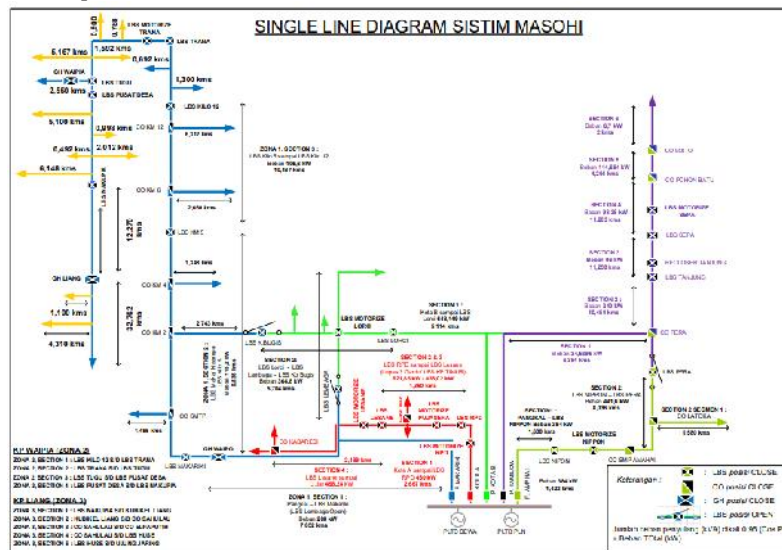
Single Line Diagram Sistim Masohi
