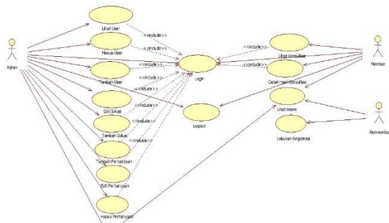
Gambar 2. UseCase Diagram
