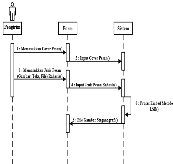
Gambar 9. Sequential Diagram Proses Embed Aplikasi Steganografi
