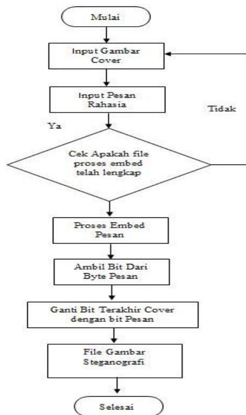
Gambar 4. Flowchart Embed Pesan Rahasia
