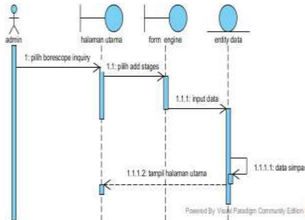
Gambar 6. Sequence Diagram
