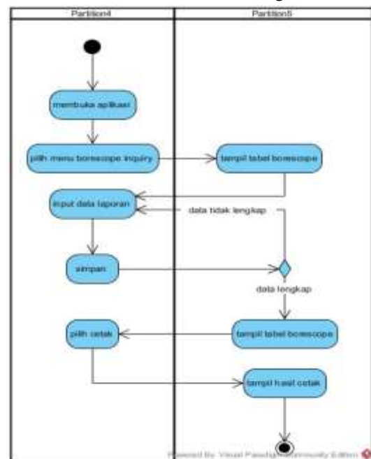
Gambar 5. Activity Diagram
