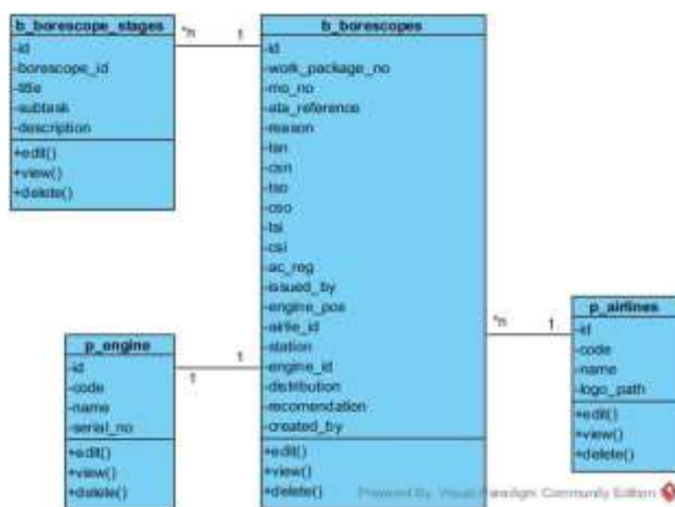
Gambar 7. Class Diagram
