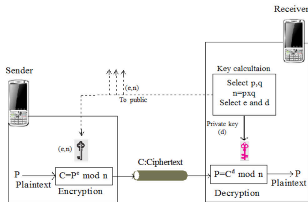
Figure 2. Encryption, decryption and key generation in RSA
