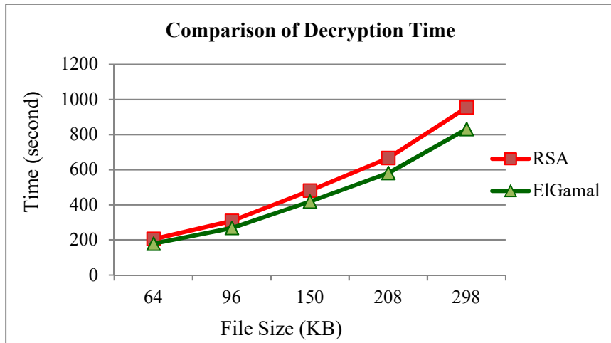
Figure 5. RSA and ElGamal decryption time comparison
