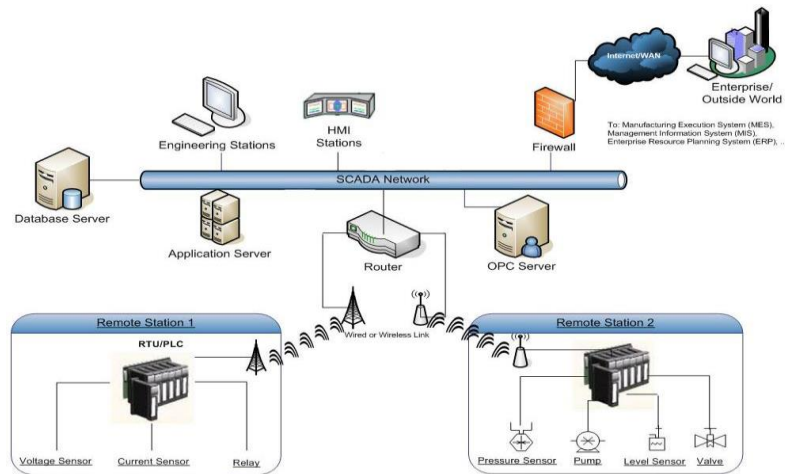
Figure 3. SCADA Network
