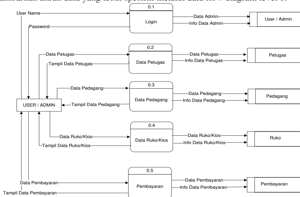
Gambar 5. Data Flow Diagram Level 0
