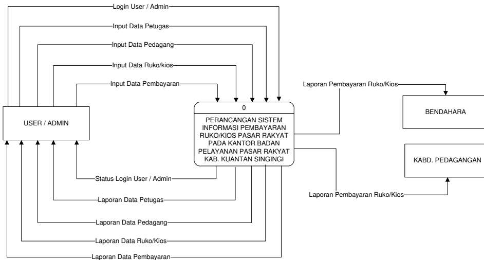
Gambar 4. Context Diagram
