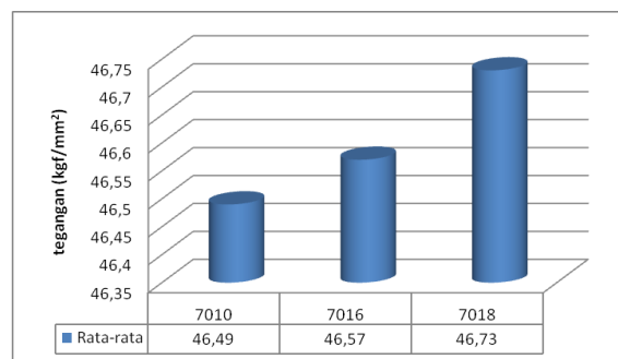
Gambar 9. Diagram Tegangan Tarik Material SS400
