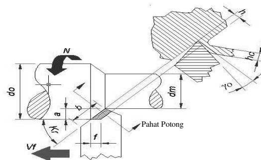
Gambar 1. Proses Bubut[2]
