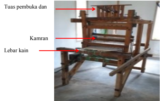
Figure 3. Loom machines
