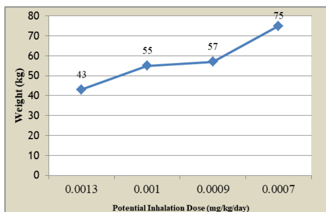
Figure 1. Potential inhalation dose of paraquat exposure
