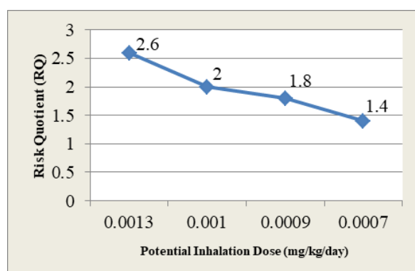
Figure 2. Risk quotient of paraquat inhalation dose at palm oil plantation
