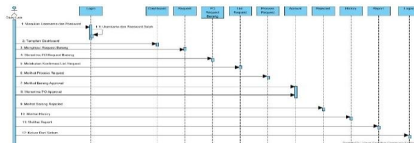
Gambar 7. Sequence Diagram Divisi Lain System Monitoring Permintaan Perlengkapan Peralatan Kantor
