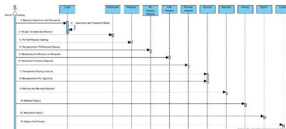
Gambar 8. Sequence Diagram Admin Purchasing System Monitoring Permintaan Perlengkapan Peralatan Kantor
