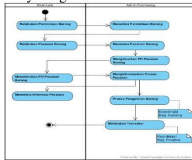
Gambar 2. Activity Diagram Monitoring Permintaan Perlengkapan Peralatan Kantor
