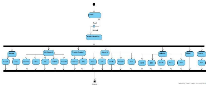
Gambar 5. Activity Diagram Admin Purchasing Sistem Monitoring Permintaan Perlengkapan Peralatan Kantor
