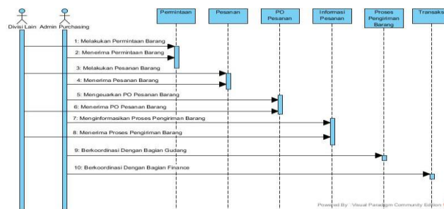
Gambar 3. Sequence Diagram Monitoring Permintaan Perlengkapan Peralatan Kantor
