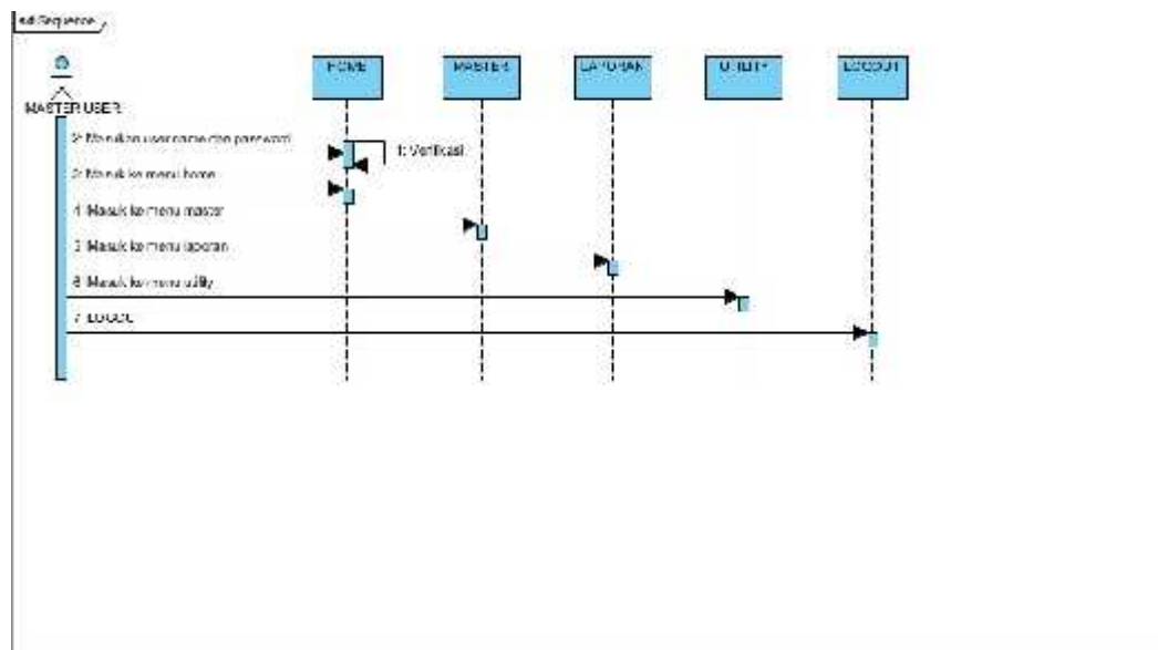
Gambar 4. Sequence Diagram
