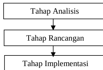
Gambar 1. Metode penelitian
