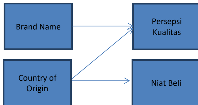
Gambar I Model Penelitian
